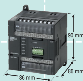
CP1L-L20D
