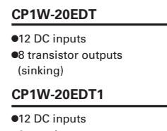
CP1W-20EDT
