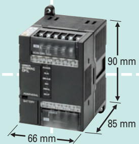
CP1L-L10D NEW
