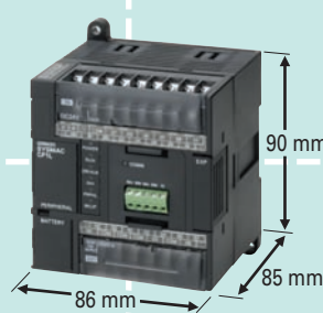
CP1L-L14D
